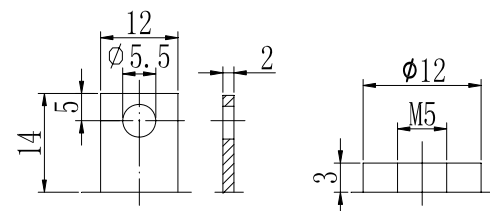
Terminal T3
